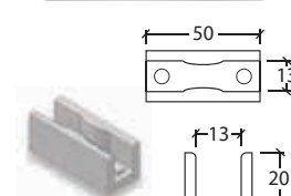
SLIDEHIDE Door-guide prevents door panel from wobbling while sliding.
