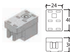
SLIDEHIDE End-stopper for positioning and preventing door panel from jumping.
