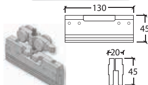
SLIDEHIDE Roller and aluminium Glass clamp. Test report is available.
