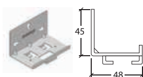
SLIDEHIDE Wall-bracket for mounting track to side of wall.
