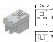
SLIDEHIDE End-stopper for positioning and preventing door panel from jumping.
