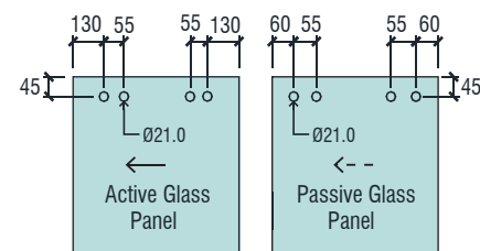
GLASS DOOR AND GLASS CLAMP HOLE DIMENSION
