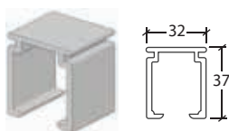
SLIDEHIDE aluminium track.
