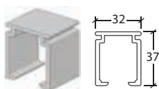
SLIDEHIDE aluminium track.
