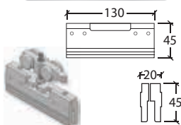
SLIDEHIDE Roller and aluminium Glass clamp. Test report is available.
