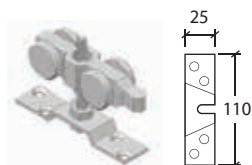
SLIDEHIDE Roller and steel Hanging-bracket. Test report is available.
