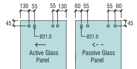
GLASS DOOR AND GLASS CLAMP HOLE DIMENSION
